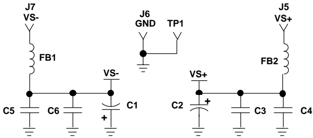
Figure 95. THS4211/THS4215 EVM Circuit Configuration
